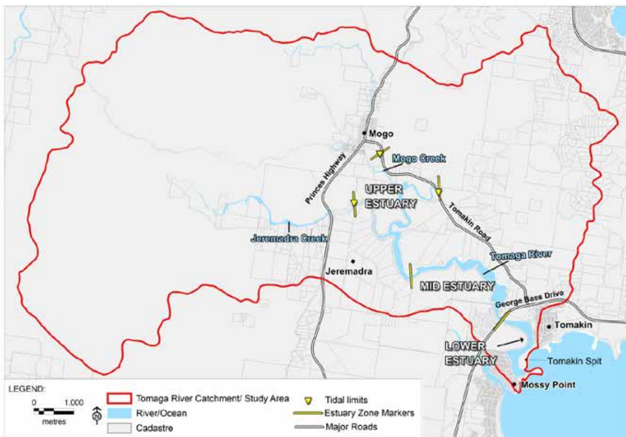
Figure 1: The Tomaga CZMP Study area (Tomaga River catchment)
