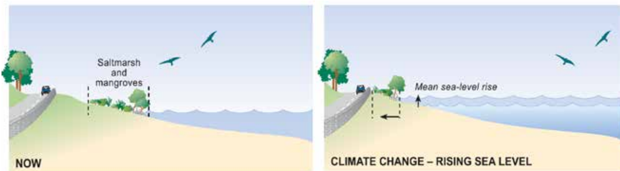
Figure 25: 'Coastal squeeze' under sea level rise: impact of development
