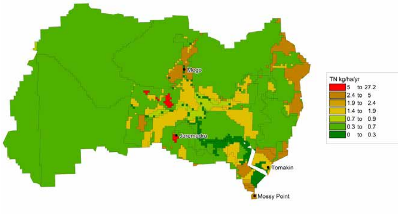
Figure 9: Modelled TN load
