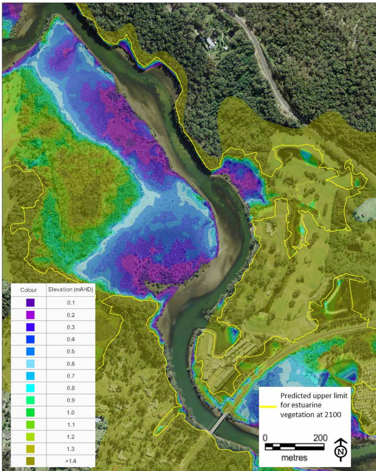
Figure 27: Potential areas for migration of estuarine vegetation types with sea level rise – mid estuary
