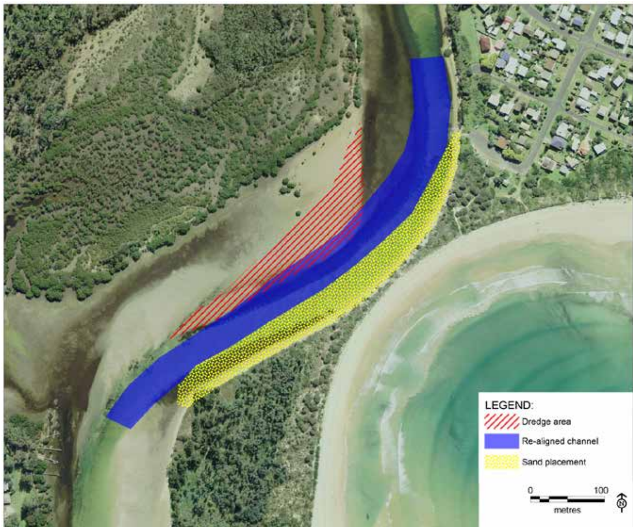
Figure 57: Option 1M – dredging of shoal and realignment of channel
