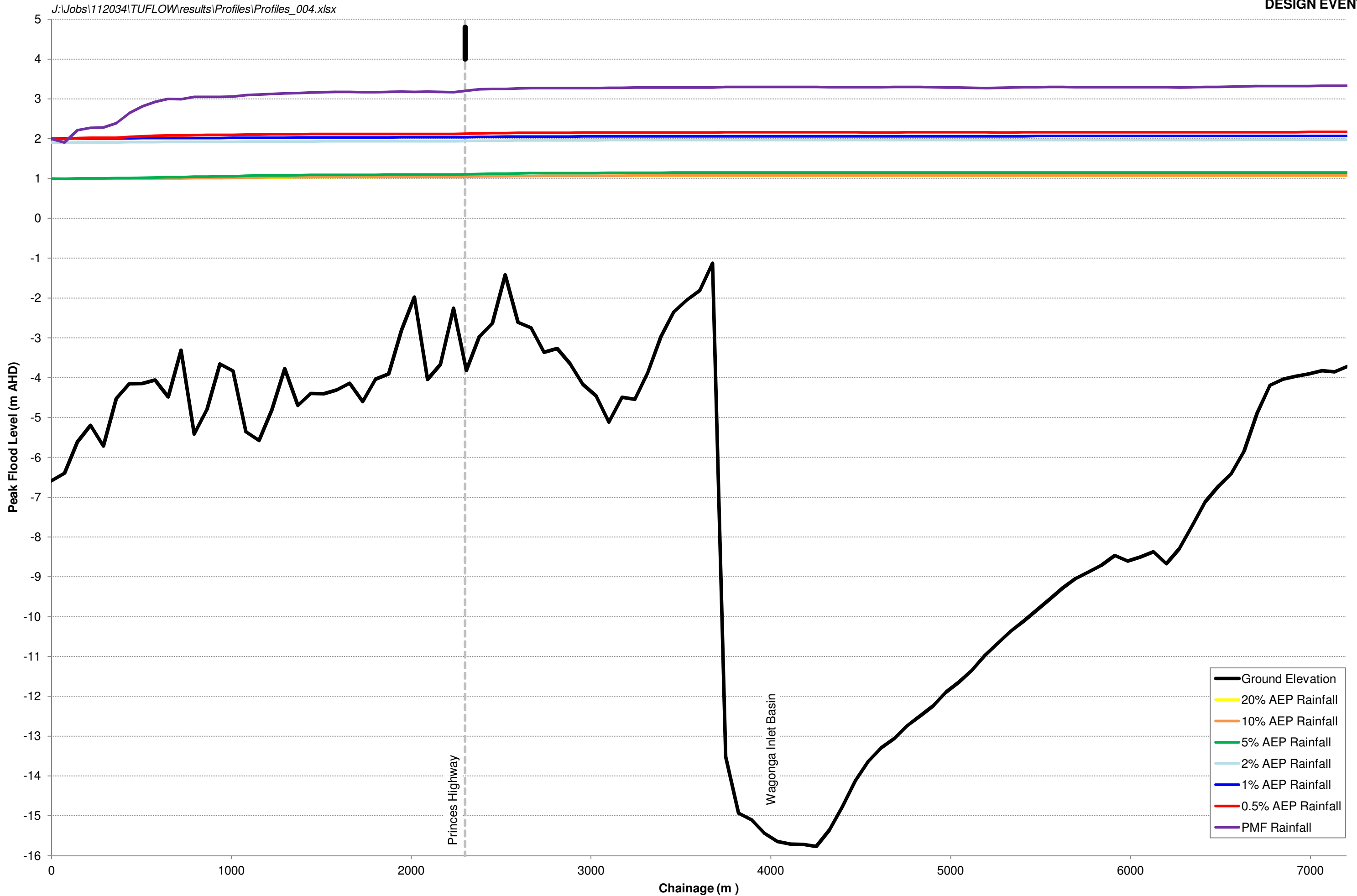
FIGURE F3 WAGONGA INLET CATCHMENT PEAK FLOOD LEVEL PROFILES DESIGN EVENTS
