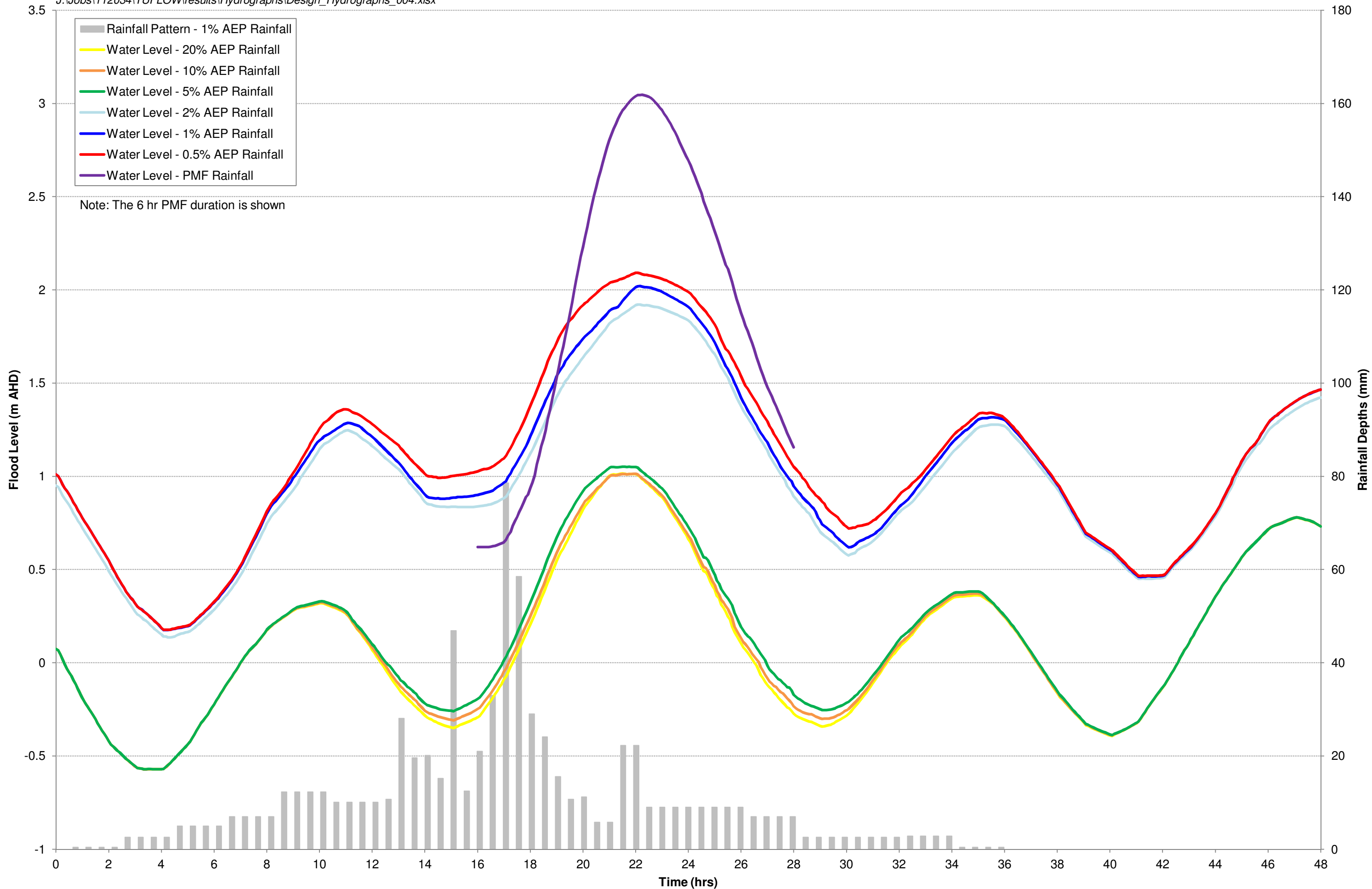
FIGURE F4B WAGONGA INLET CATCHMENT FLOOD LEVEL HYDROGRAPHS NAROOMA PUBLIC WHARF
