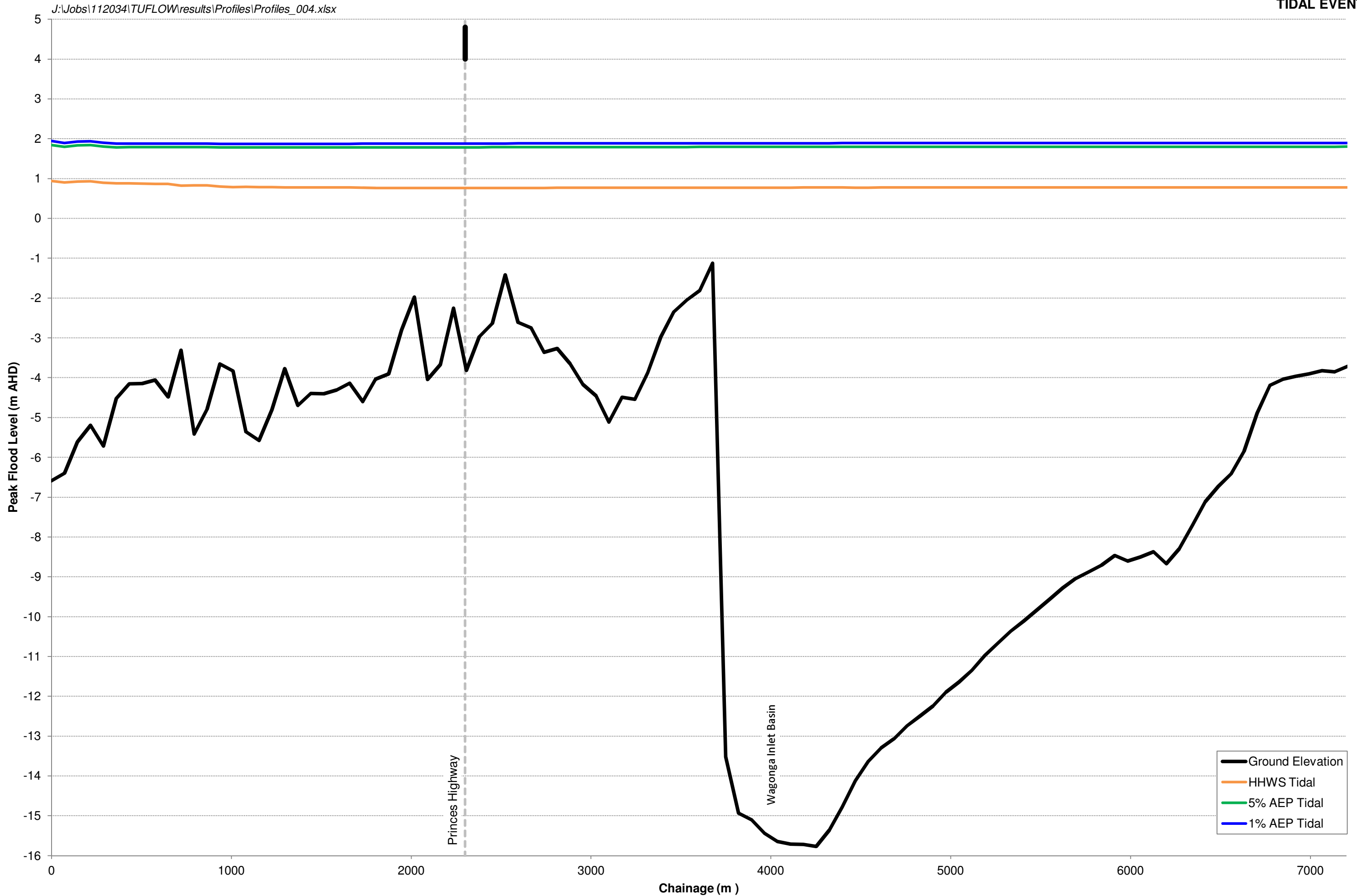
FIGURE F2 WAGONGA INLET CATCHMENT PEAK FLOOD LEVEL PROFILES TIDAL EVENTS
