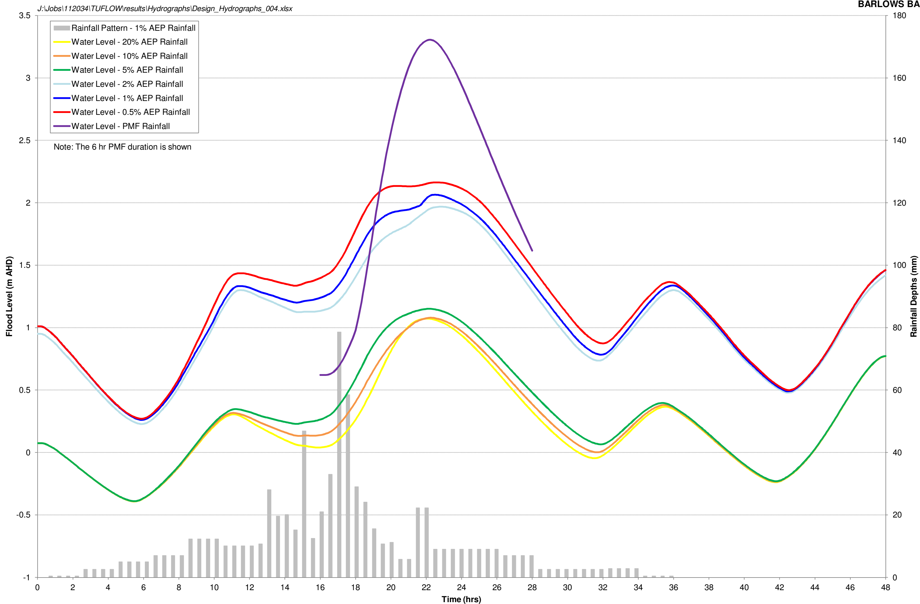
FIGURE F4A WAGONGA INLET CATCHMENT FLOOD LEVEL HYDROGRAPHS BARLOWS BAY
