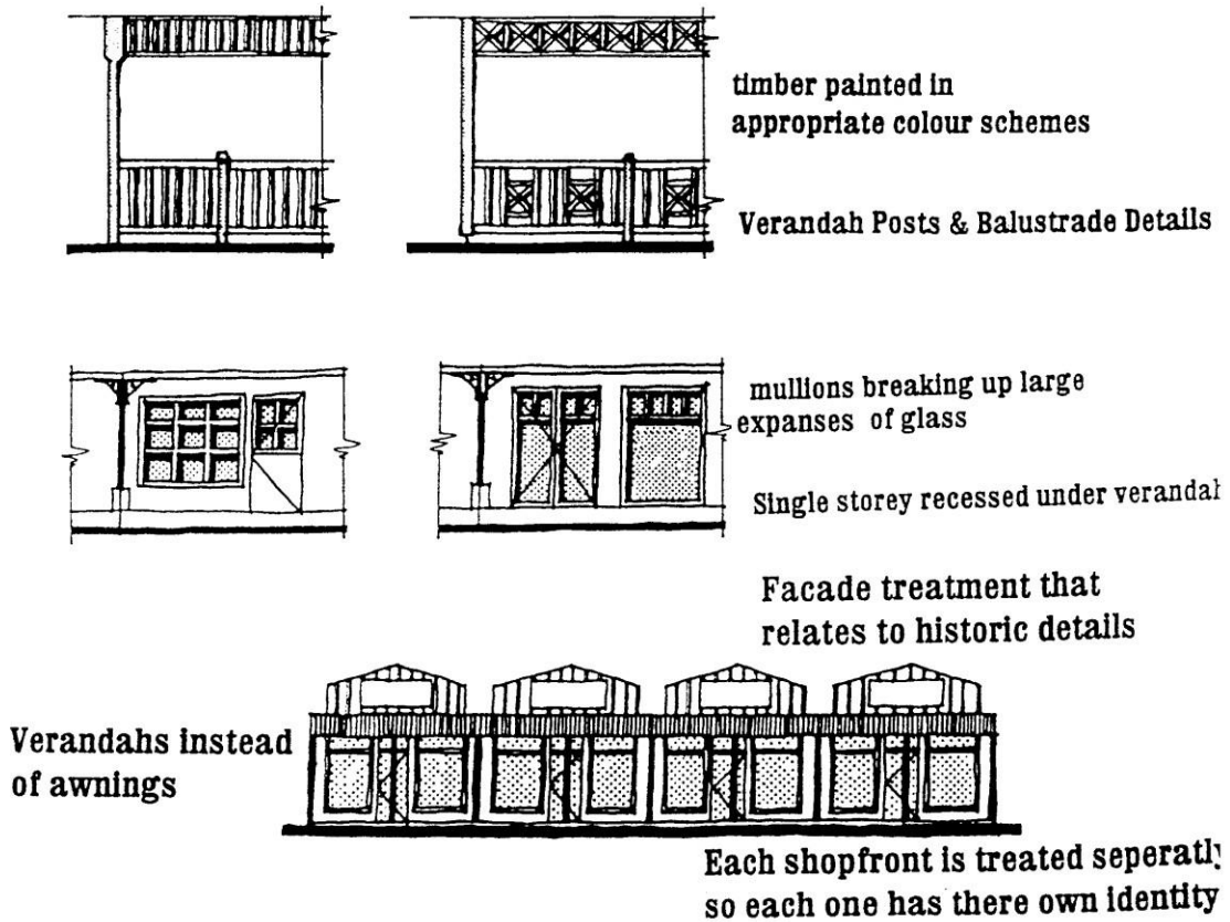
Figure 2: Examples of design and façade articulation which enhances the historic theme
