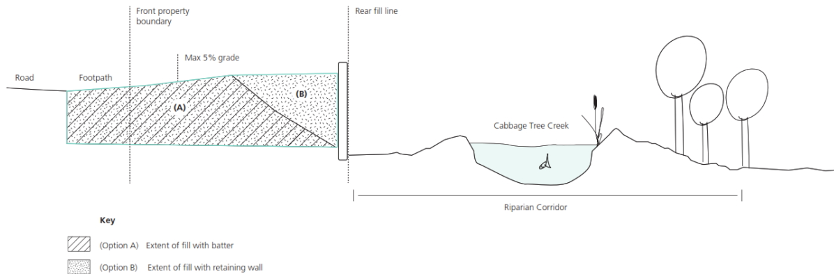
FIGURE 6: Example fill options diagram (not to scale)
